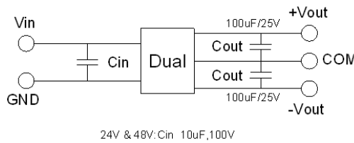
Recommended Test Circuit
