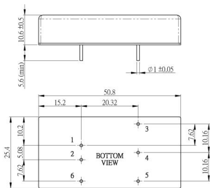
Markings and dimensions
