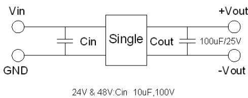
Recommended Test Circuit
